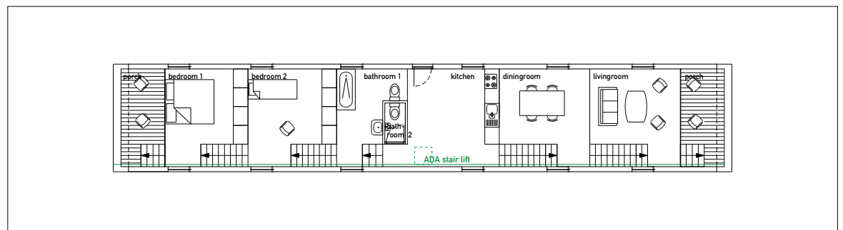
floorplan
